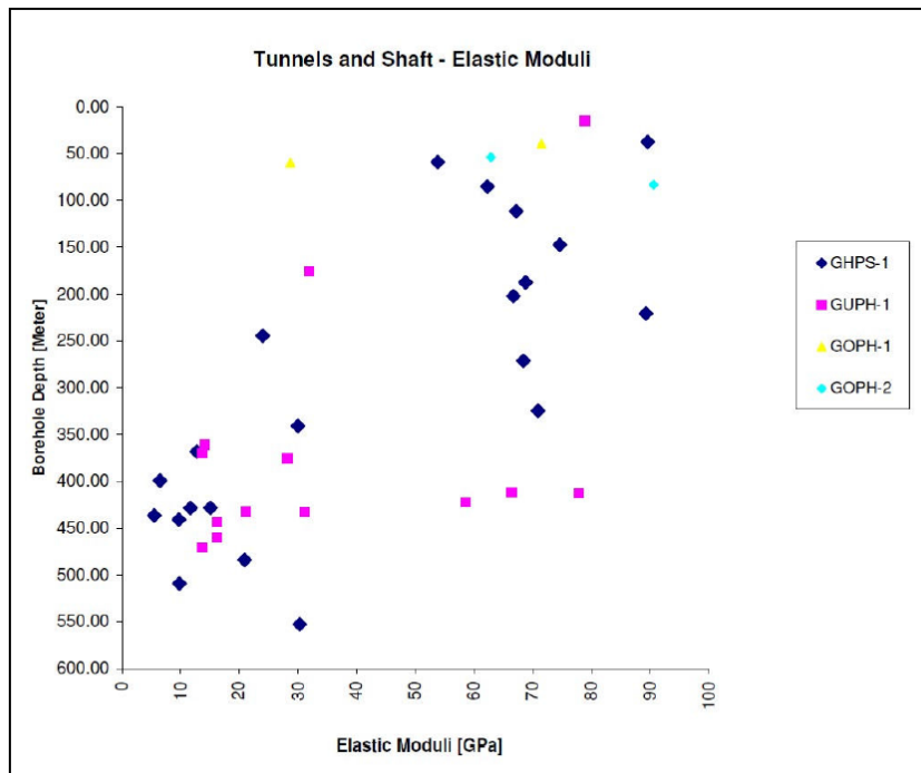
Fig. 5: Distribution of the Elastic modulus with borehole depth (intact rock)
